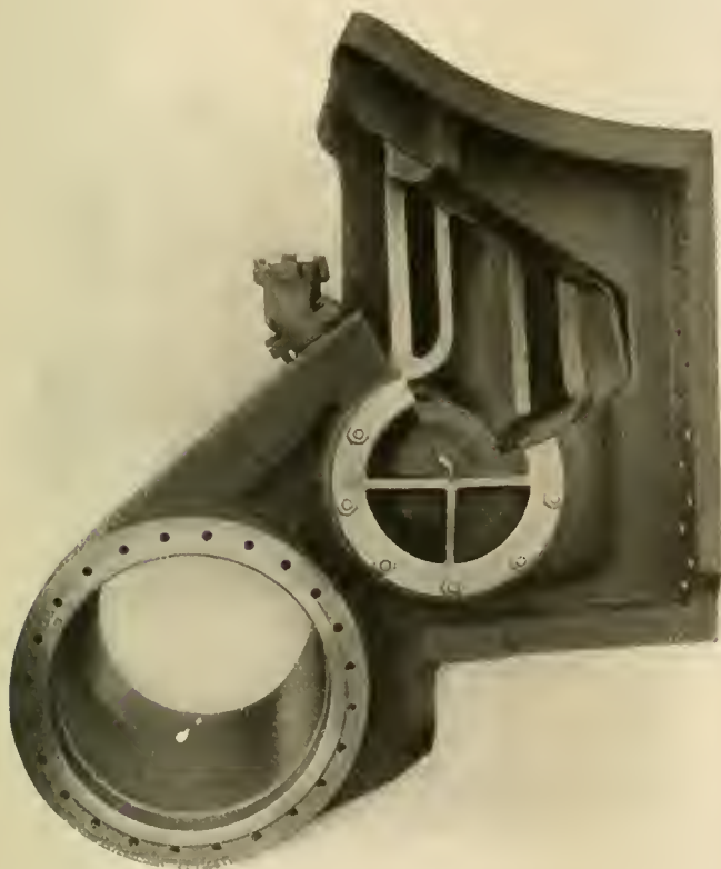
FIG. 1.—CYLINDER AND PISTON VALVE
